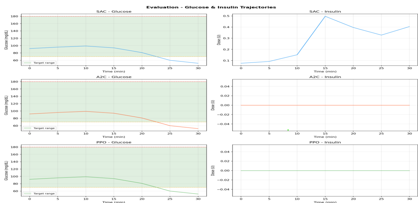
Figure 5: Representative glucose and insulin dose trajectories during policy evaluation for SAC, A2C, and PPO
