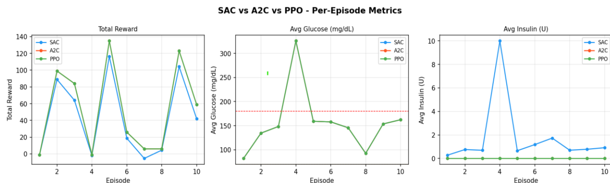
Figure 3: Per-episode total reward, average glucose, and average insulin dose for SAC vs. A2C across 10 evaluation episodes.
