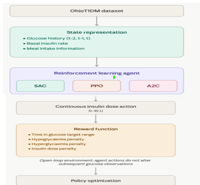
Figure 1: Overview of the proposed reinforcement learning framework for personalized insulin dosing, showing the interaction between the open-loop environment, the RL agent (A2C, SAC, or PPO), and the reward function.
