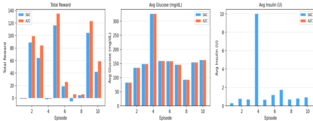
Figure 4: Comparison of cumulative reward, average glucose, and average insulin dose for SAC, A2C and PPO
