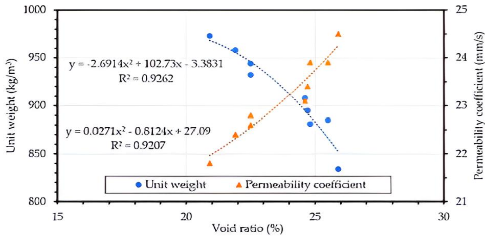
Figure-4: Unit weight and permeability coefficient versus void ratio (Tang et al., 2022).
