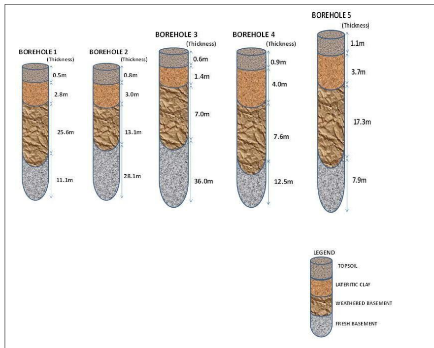
Figure 4: Borehole lithologic logs
