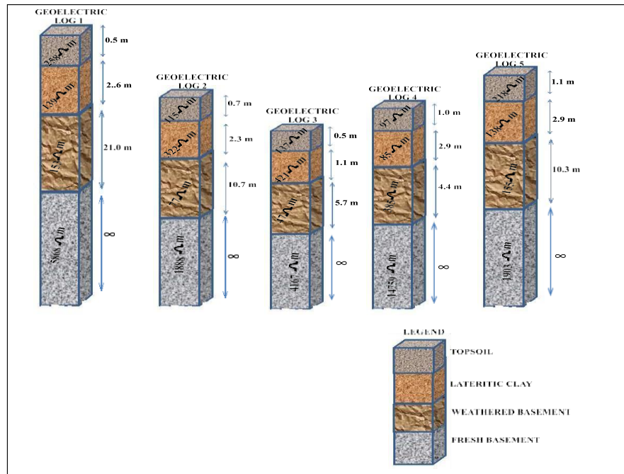
Figure 3: Geoelectric logs
