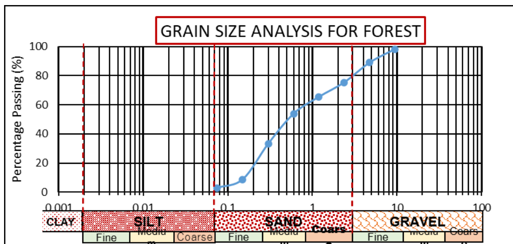
Figure 10: Grain size graph for Forest
