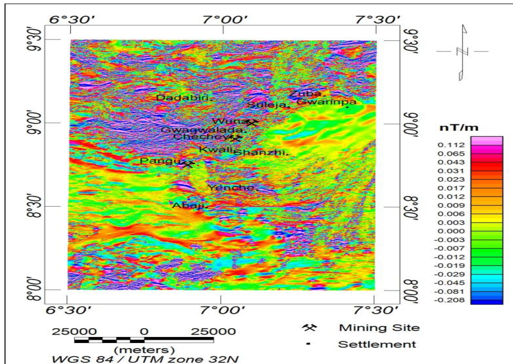
Fig. 6: First Vertical Derivative map of the study
