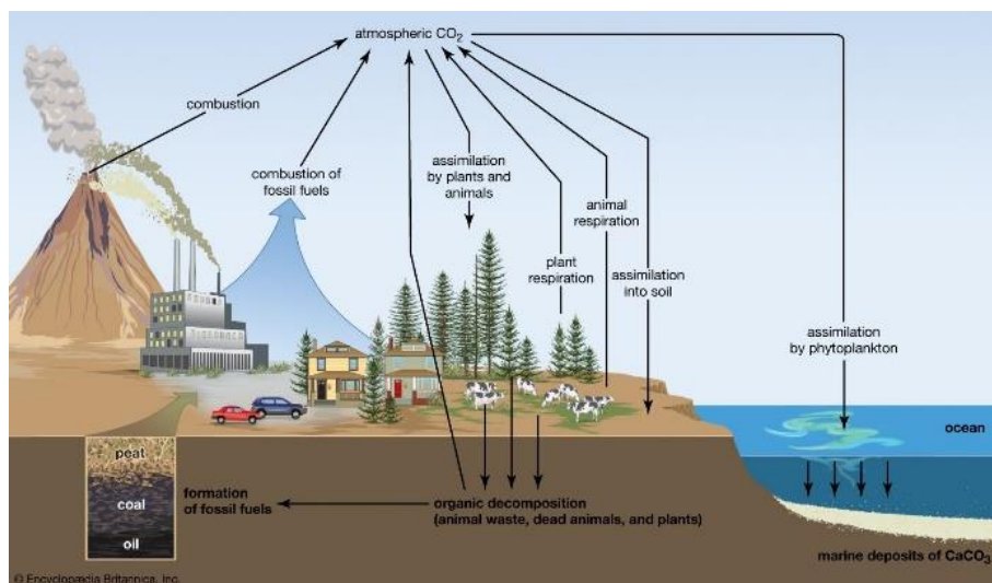
Figure 1. Carbon cycle. 8
