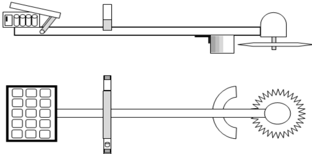
Figure 4 the skeletal design of Solar powered E-grasscutter
