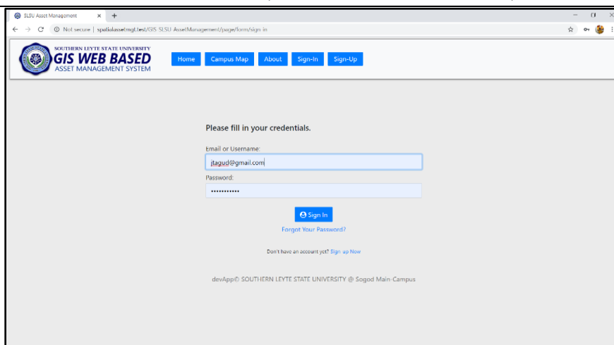
Fig. 4 Log-in Page
