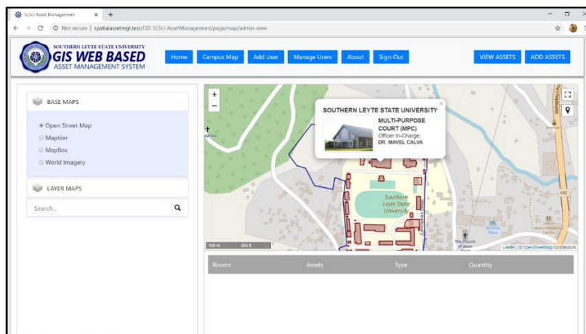
Fig. 5 Campus Page
