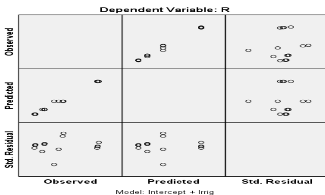
Fig 6: Residual Plots for R
