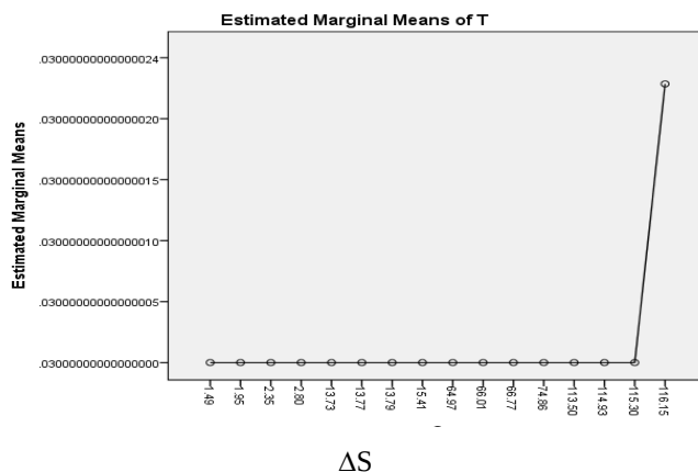
Figure 5: Estimated Marginal Means for T
