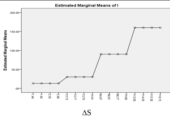
Fig 1: Estimated Marginal Means for I
