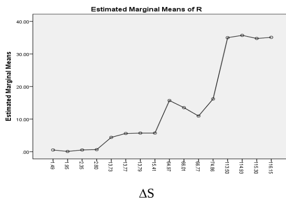
Fig 2: Estimated Marginal Means for runoff (R)
