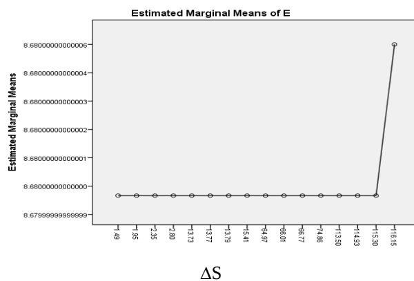
Fig 4: Estimated Marginal Means for (E)
