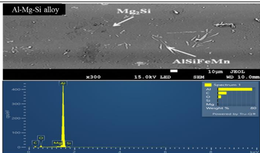
Fig. 3 SEM-EDS micrograph of Al-Mg-Si alloy as-cast
