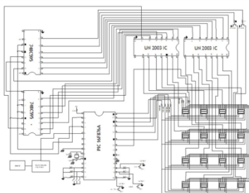
Fig. 6. Circuit Diagram of Controll Section
