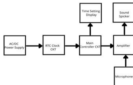
Fig. 2. Block Diagram of the Proposed System.
