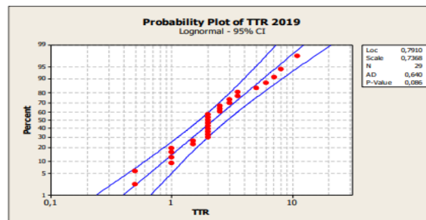
Fig.4. 2020 Goodness of Fit Time To Failure Test
