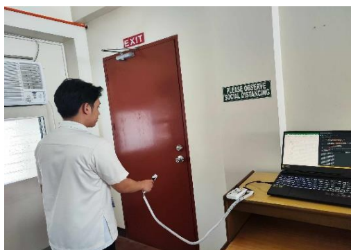
Fig 9. Testing of Smart Stick Detection on Wood
