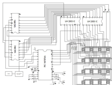
Fig. 6. Circuit Diagram of Controll Section
